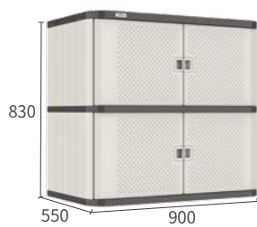
TPL-B900S1 Two-story
